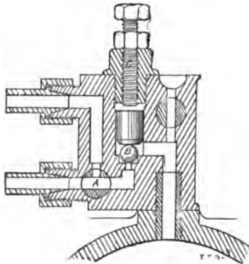
FIG. 293.—The "Lombard" Improved Cylinder Cooling Device. Instead of wing flanges, or jacket water, this system provides for cooling the cylinder by injection of a small quantity of water, atomized by suction of the piston. This water comes through the lower tube to the left of the cylinder head, passing through the three-way cock, A, and the ball valve, B. The lift of the ball valve is determined by the adjusting screw, C. When water is not required, the three-way cock is turned so as to return it to the tank through the upper left-hand tube. The theory is that superfluous heat will be absorbed in vaporizing the injected water.
